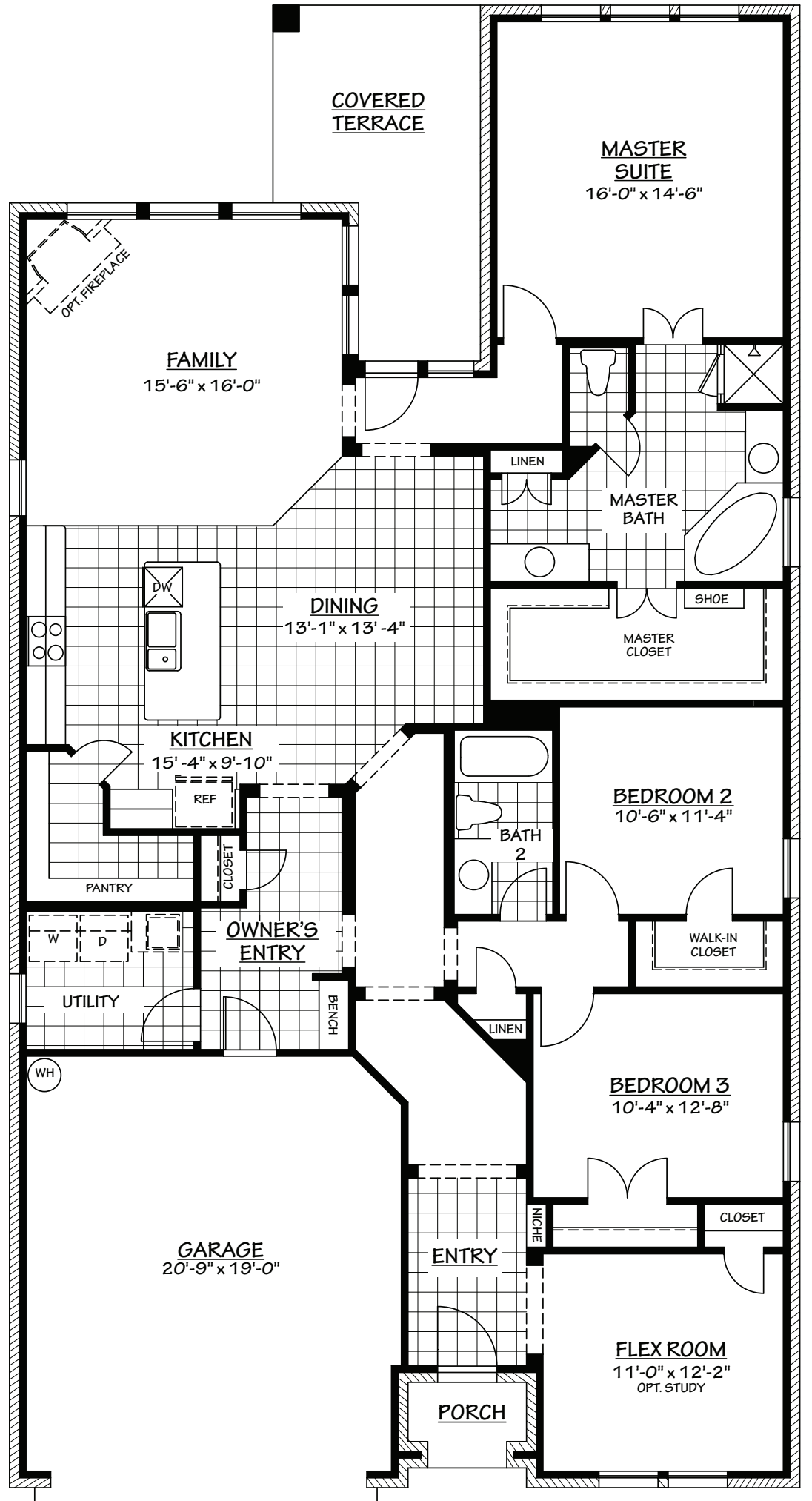
FLOOR PLAN
